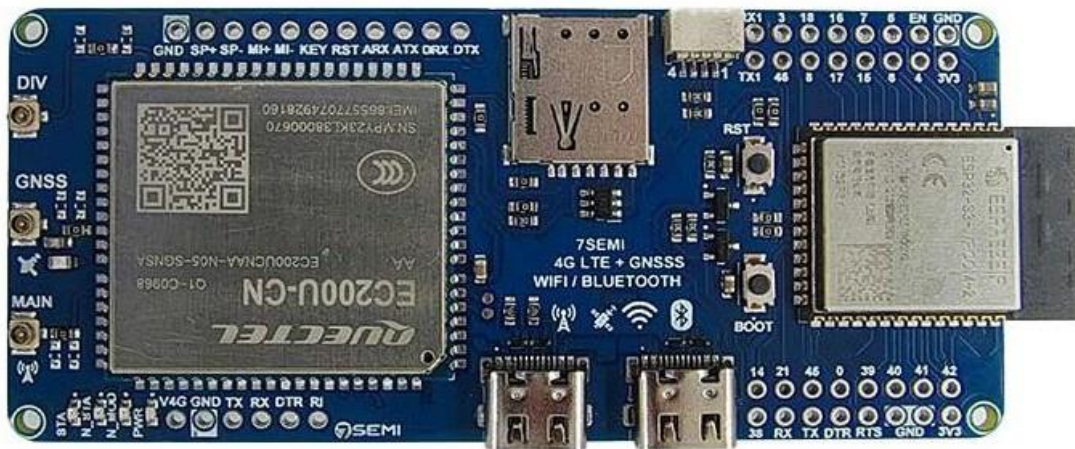
Figure 2.1.3 Top view
