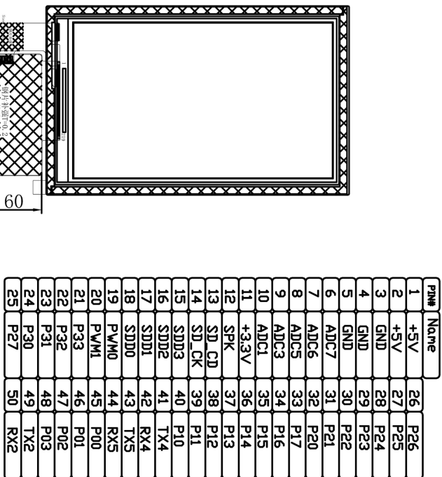
LCD PIN
