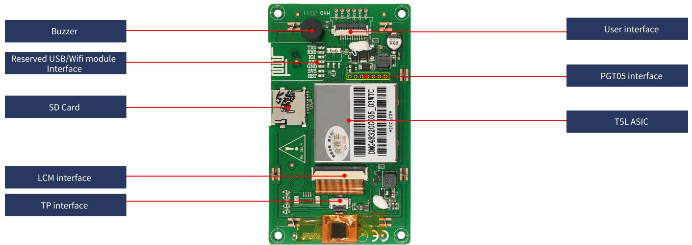
Hardware interface
