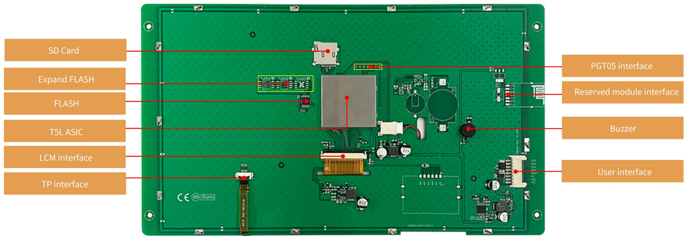
Hardware interface
