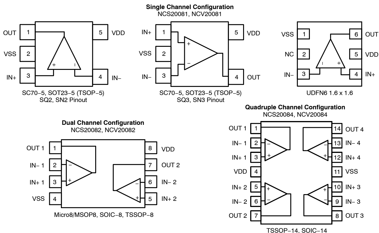
Figure 1. Pin Connections
