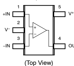
SC70-5/TSOP-5
