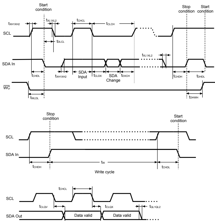
Figure 17. AC waveforms
