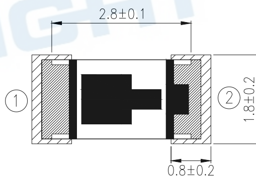
Recommend Soldering Pad
