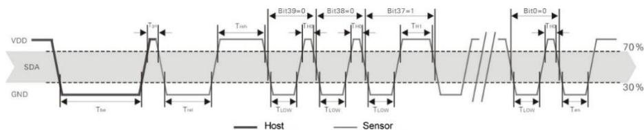
Figure 9. AM2305B Single bus communication timing
