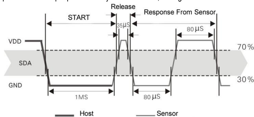
Figure 10. Single Bus Decomposition Timing Diagram
