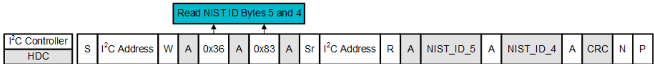
Figure 7-29. I 2 C Command Sequence: Read NIST ID (Bytes NIST_ID_5, Then NIST_ID_4)
